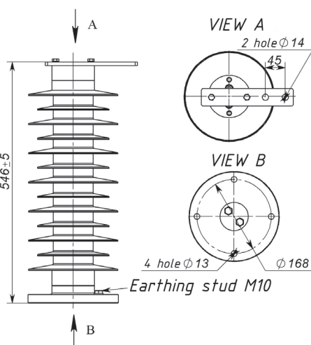
Fig. 27 Type of housing 356
