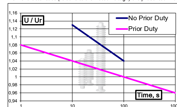
Fig. 5 TOV characteristics
