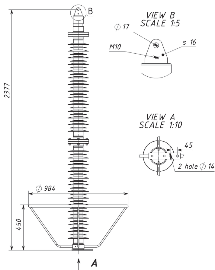
Fig. 39 Type of housing 301- -1/3
