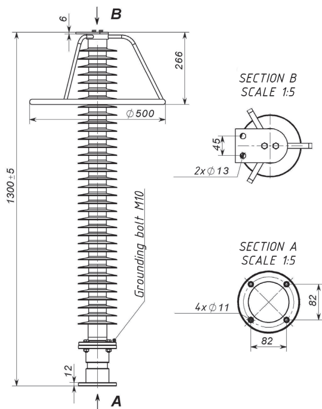
Fig. 24 Type of housing 112- -0/1
