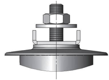
Fig. 13 High-voltage input «03» type (6 to 50 mm 2 )
