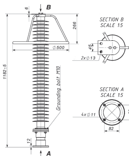
Fig. 22 Type of housing 111- -0/1
