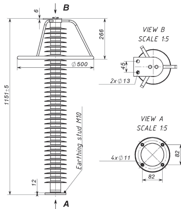
Fig. 18 Type of housing 112
