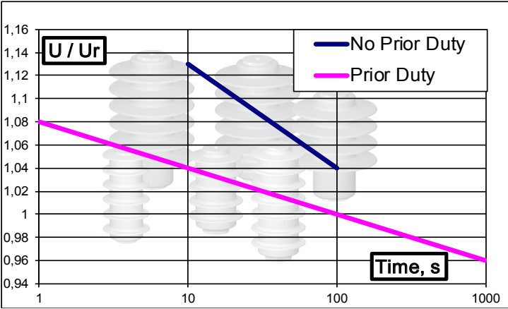
Fig. 5 TOV characteristics
