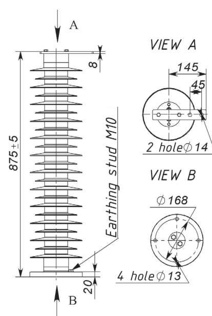
Fig. 28 Type of housing 563
