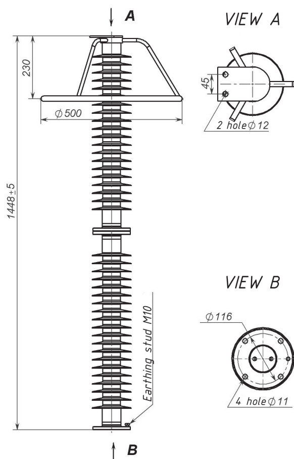
Fig. 19 Type of housing 256
