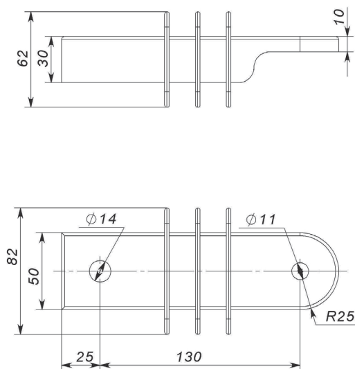
Fig. 16 Insulation bracket «I1» type. MCOV 2.55 to 15.3 kV
