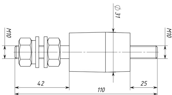
Fig. 19 D4 disconnect
