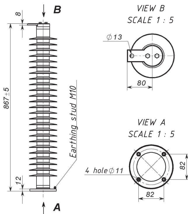
Fig. 16 Type of housing 562
