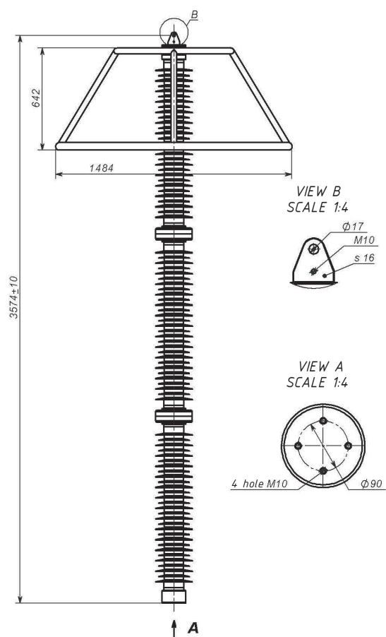
Fig. 37 Type of housing 302- -0/2
