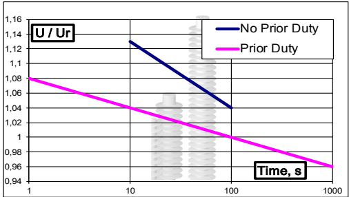
Fig. 5 TOV characteristics
