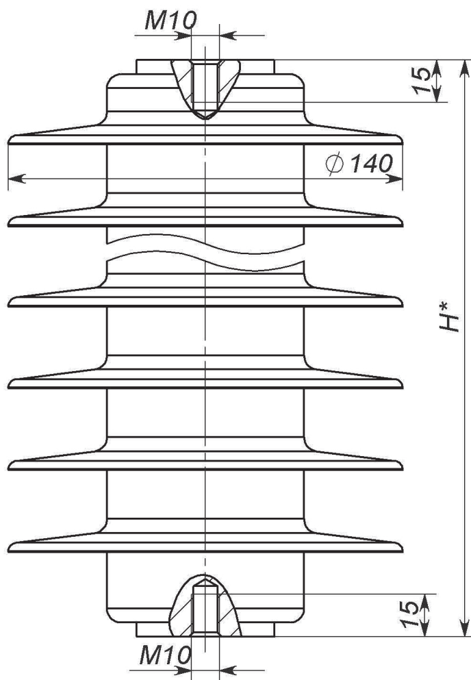
Fig. 11 PA-DH-151, 152, 203, 204, 351
